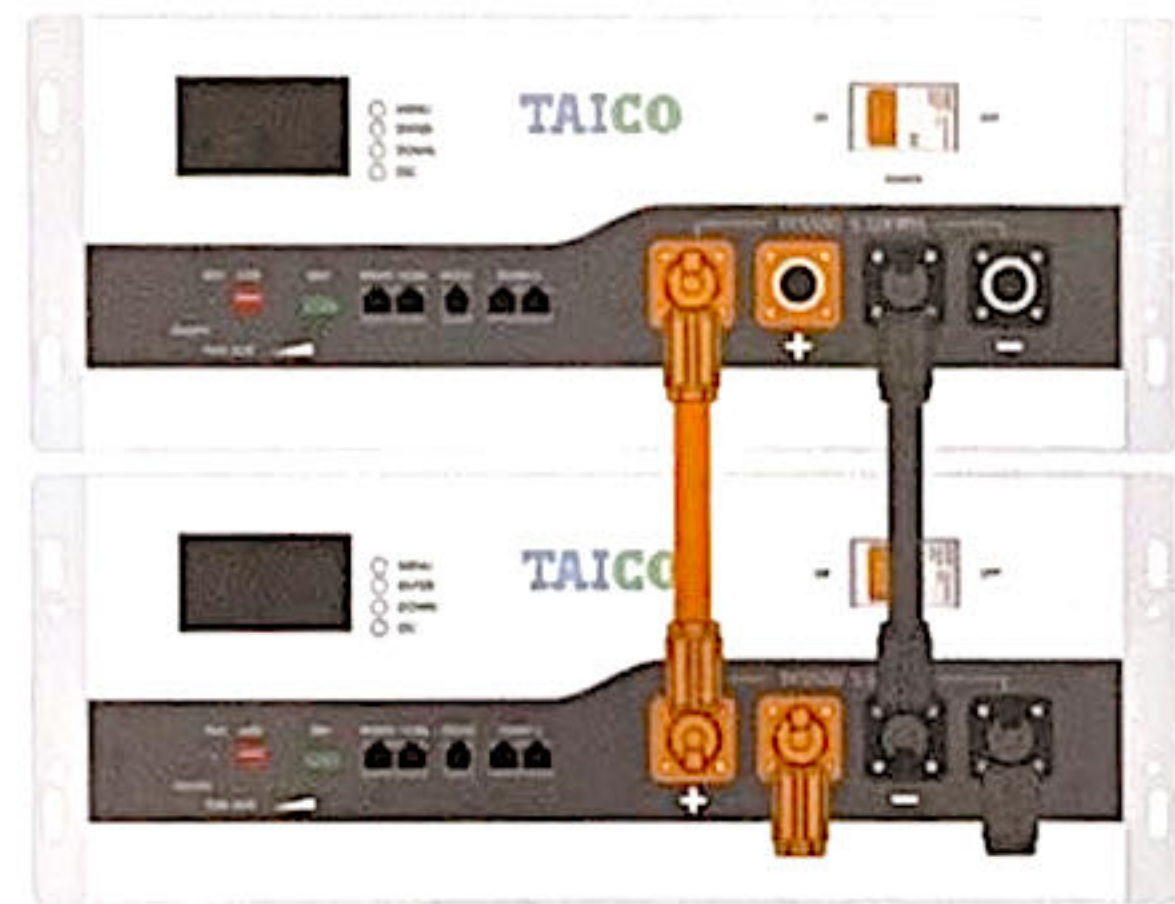
Two batteries installed
