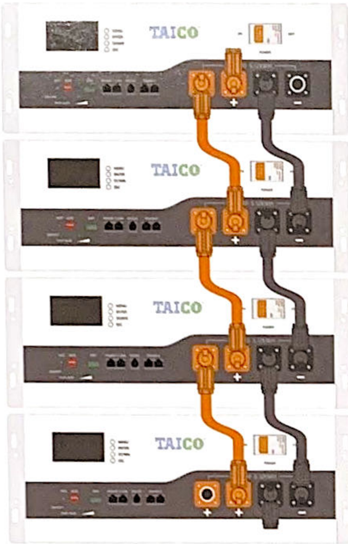
Four batteries installed
