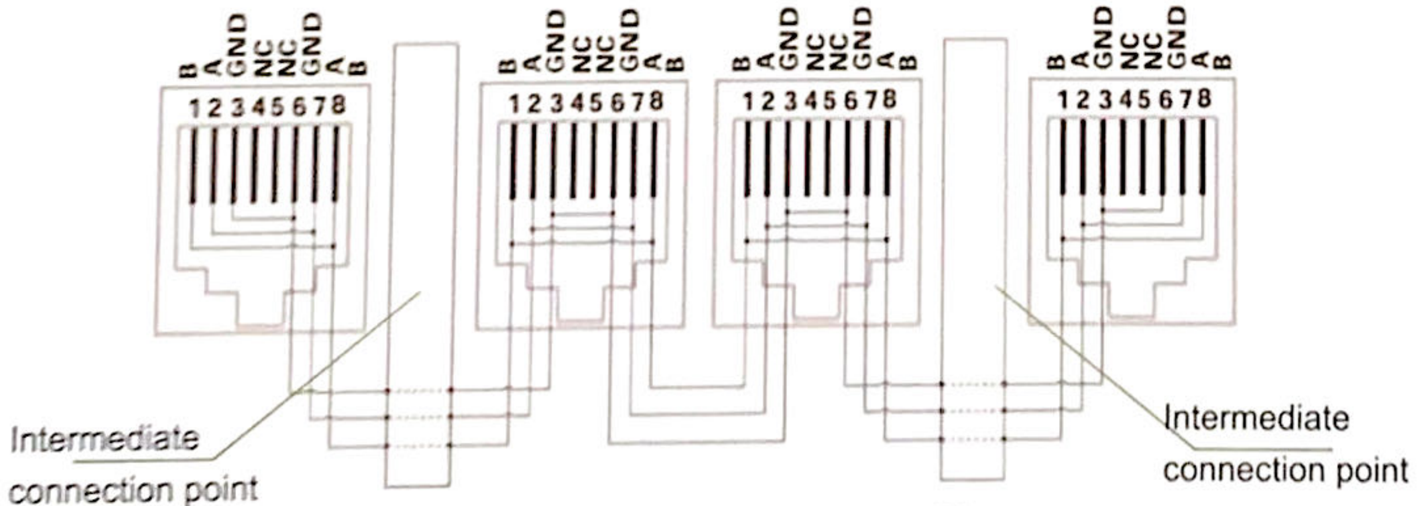
RS485 Parallel Connection Diagram
