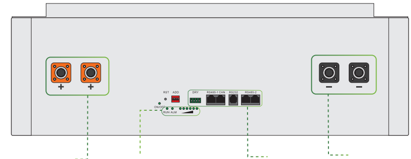
Power Cable Interface Indicator light Communicate terminals Power Cable Interface
